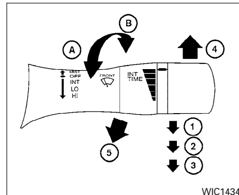
SWITCH OPERATION
