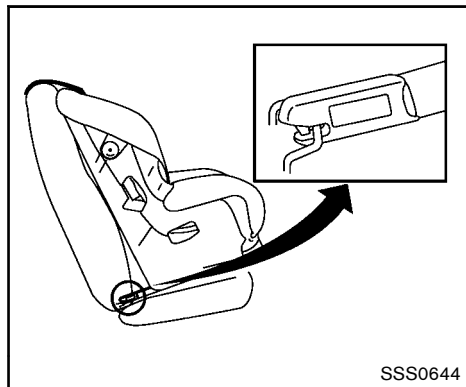
LATCH rigid-mounted
